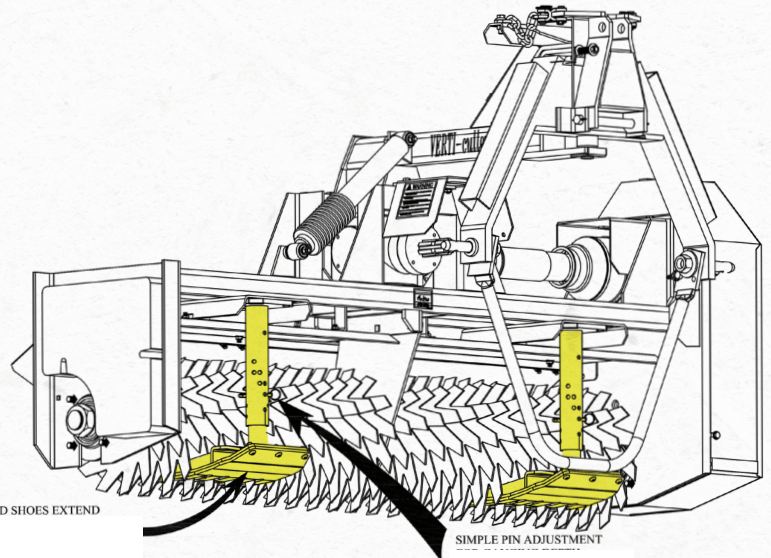
Skid shoes extend between blades for consistent cutting depth over uneven turf
