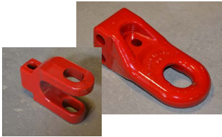
PPI-301 With Clevis & V Block Available on 400T-800T
